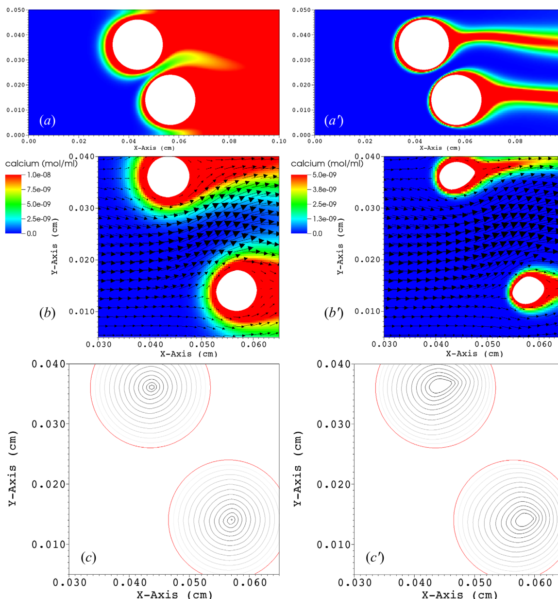
Figure 4. Results for the two-grain simulations at two prescribed inlet fluid velocities: (a, b, c) v = 0.012 cm/s and (a', b', c') v = 0.12 cm/s. (a, a') Calcium concentrations at steady state conditions for reactive transport with the initial grain size, in the entire simulation domain. (b, b') Calcium concentrations at steady state conditions for reactive transport at later stages of grain evolution (673 h in Figure 4b and 606 h in Figure 4b'), with vectors showing local fluid velocities and relative magnitudes, in the pore throat region of the domain. (c, c') Evolution of the grain surfaces with time: in red is the initial grain boundary, and later stages are shown as a gray scale with increasing shade with time.
