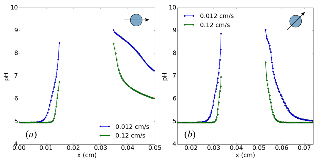
Figure 3. pH values plotted along (a) a horizontal line and (b) a line at 45° with the horizontal, for two flow conditions, showing the thickness of the local diffusive boundary at steady state conditions for reactive transport with the initial grain size (i.e., Figure 1, left). The gap in values indicates the presence of the mineral grain.
