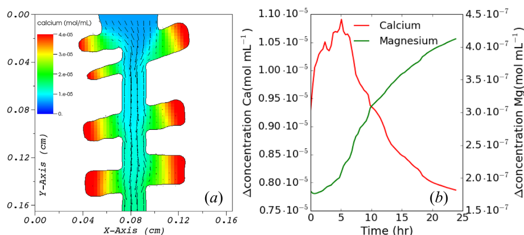
Figure 11. (a) Simulated fracture geometry at 24 h showing calcium concentrations within the fracture aperture and local flow velocities in arrows. (b) Changes in effluent calcium and magnesium concentrations over time.
