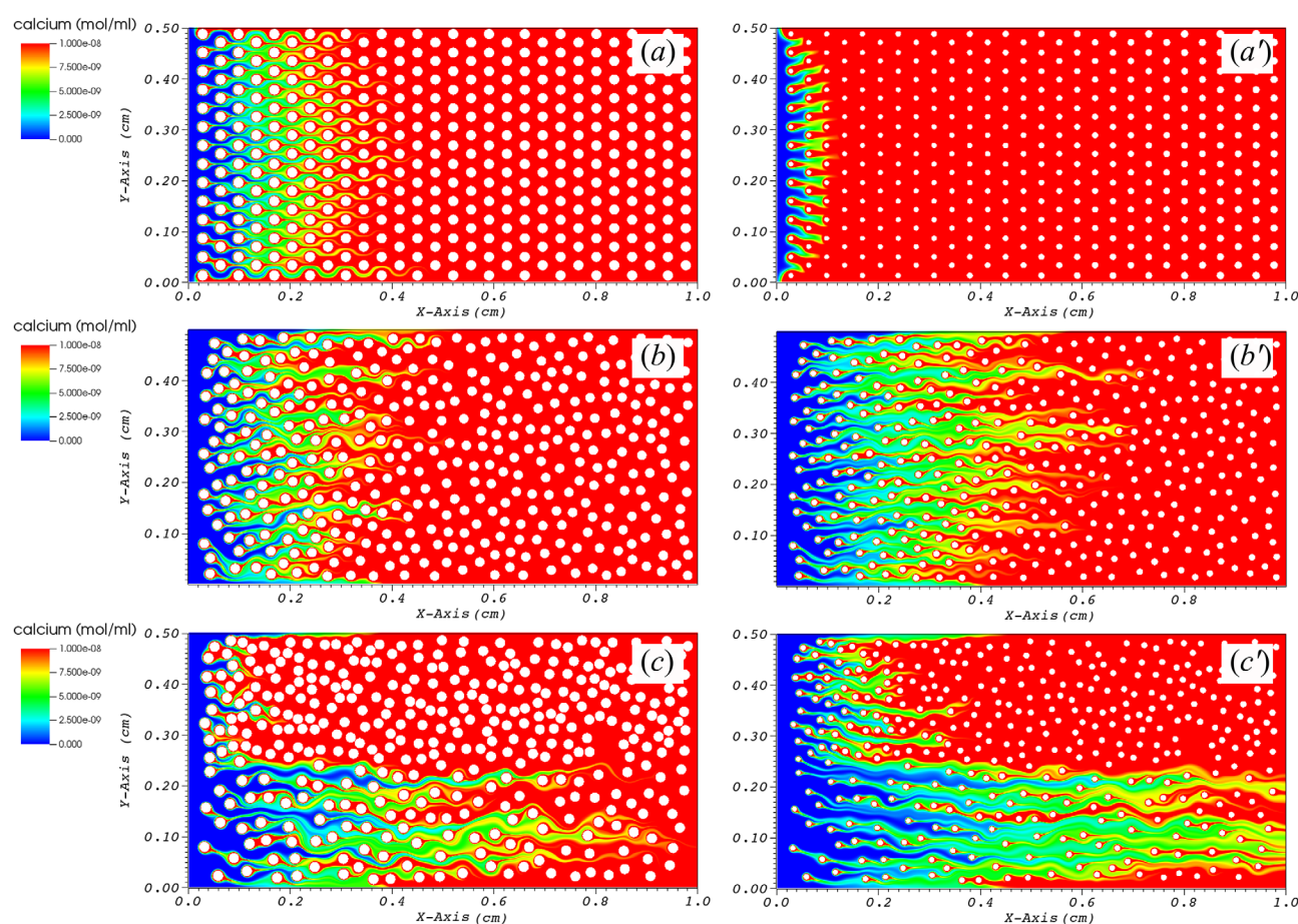
Figure 5. Calcium concentrations at steady state conditions for reactive transport for a prescribed inlet fluid velocity of 0.12 cm/s in three grain packings: (a, a') uniform, (b, b') heterogeneous and (c, c') two-zone packing. Figures 5a–5c show conditions that correspond to the initial geometry, and Figures 5a'–5c' show a later stage of the evolution, namely, t = 576 h, 588 h, and 468 h, respectively.
