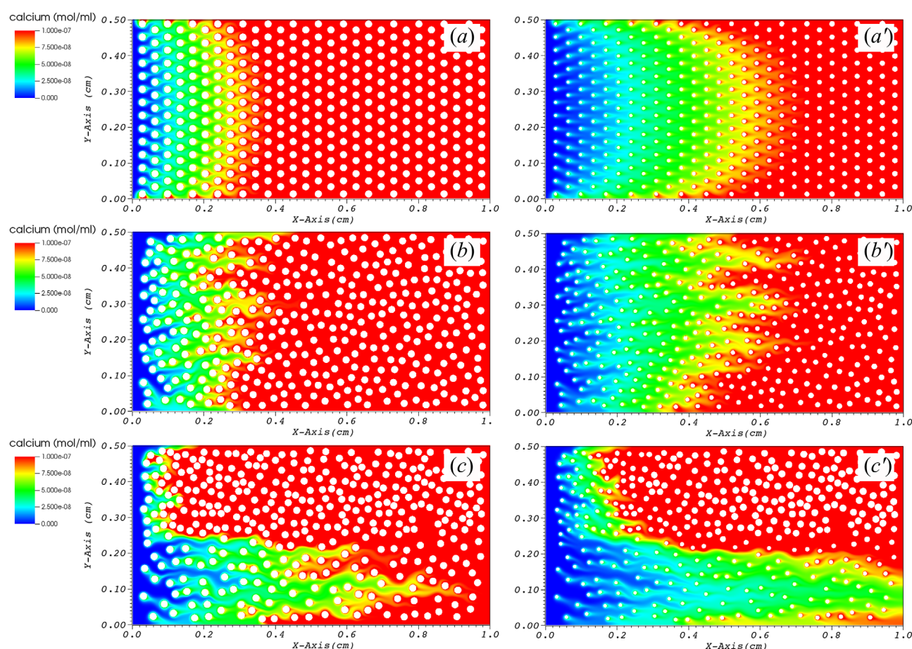
Figure 6. Calcium concentrations at steady state conditions for reactive transport for a prescribed inlet fluid velocity of 0.012 cm/s in three grain packings: (a, a') uniform, (b, b') heterogeneous, and (c, c') two-zone packing. Figures 6a–6c show conditions that correspond to the initial geometry, and Figures 6a'–6c' show a later stage of the evolution, namely, t = 639 h, 593 h, and 572 h, respectively.
