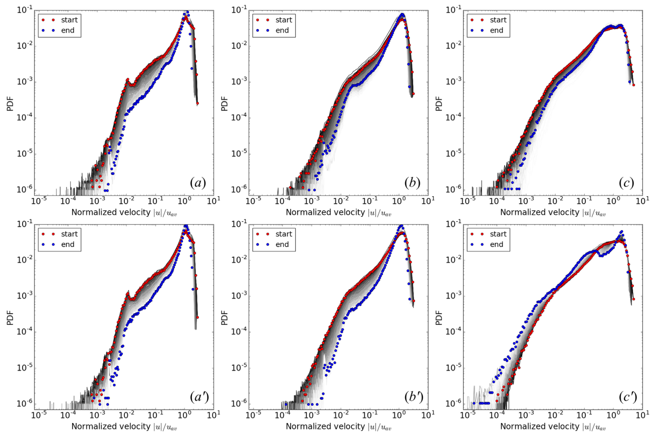
Figure 7. Initial (red) and final (blue) fluid velocity distributions in three grain packings: (a, a') uniform, (b, b') heterogeneous, and (c, c') two-zone packing. Intermediate distributions are shown as gray-scale values with intensity decreasing with time. Figures 7a–7c are for a prescribed inlet fluid velocity of v = 0.1 cm/s, while Figures 7a'–7c' are for v = 0.01 cm/s.
