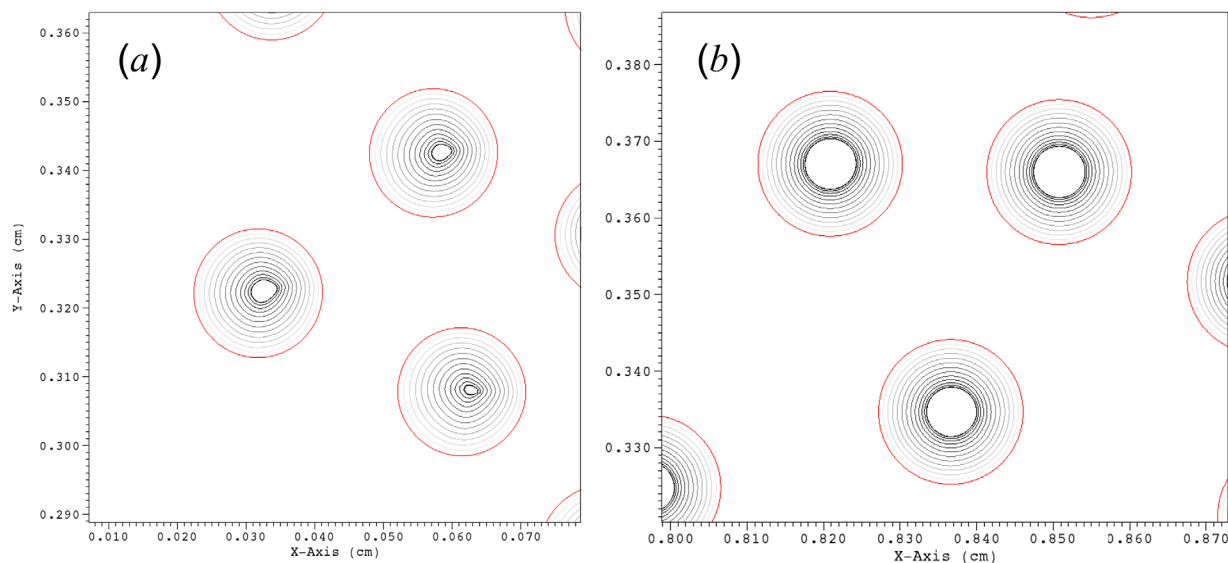
Figure 8. Evolution of the grain boundary geometry in two selected sections of the heterogeneous grain packing located (a) near the inlet and (b) near the outlet for a prescribed inlet fluid velocity of v = 0.1 cm/s. In red is the initial grain boundary; later stages are shown as a gray scale with shade increasing with time.
