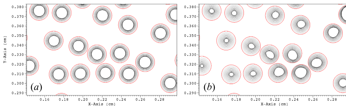
Figure 9. Evolution of the grain boundary in a selected region of the two-zone grain packing domain for a simulation with a prescribed inlet fluid velocity of (a) 0.1 cm/s and (b) 0.01 cm/s. In red is the initial grain boundary; later stages are shown as a gray scale with shade increasing with time.
