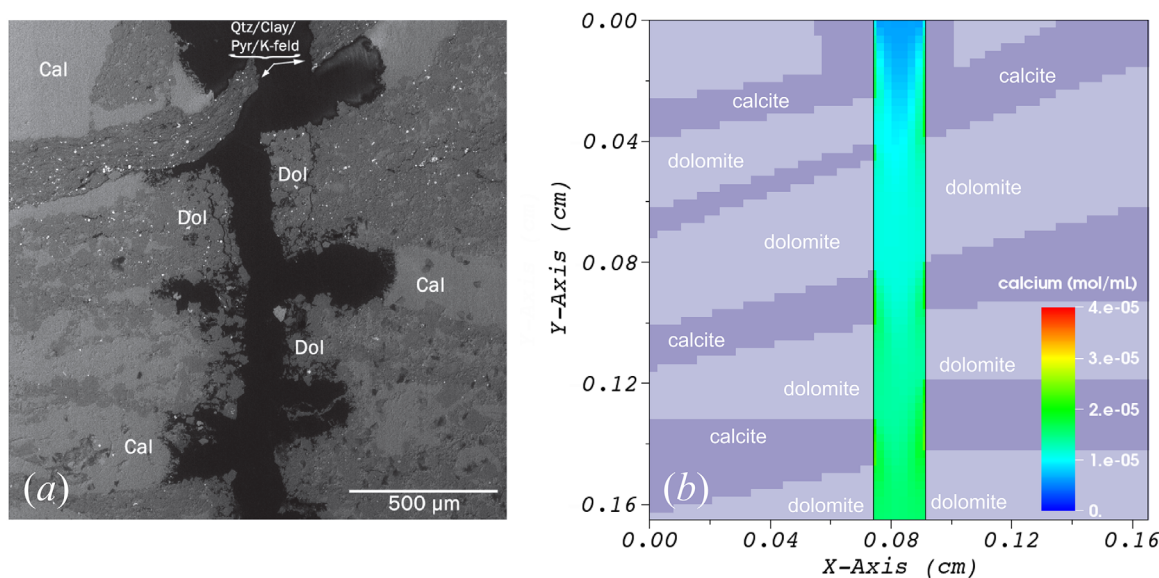
Figure 10. (a) BSE image showing preferential dissolution of calcite on a fracture surface at the end of the experiment of Ellis and coworkers [from Ellis et al. , 2011]. (b) Simulation domain in the current work showing the initial mineral composition and geometry, and the calcium concentrations in the fracture at steady state conditions for reactive transport.
