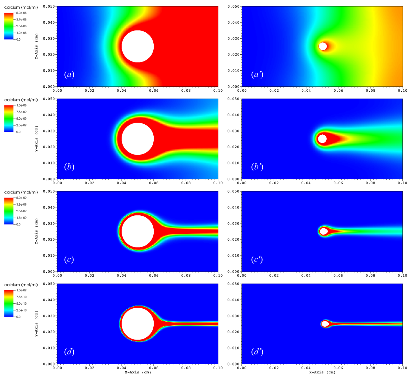
Figure 1. Calcium concentrations around a dissolving grain of calcite at steady state conditions for reactive transport for a range of prescribed inlet fluid velocities: (a, a') 0.0012 cm/s, (b, b') 0.012 cm/s, (c, c') 0.12 cm/s, and (d, d') 1.2 cm/s. Figures 1a–1d show conditions that correspond to the initial grain size, and Figures 1a'–1d' show later stages of the evolution, namely, t = 909, 820, 696, and 438 h, respectively.
