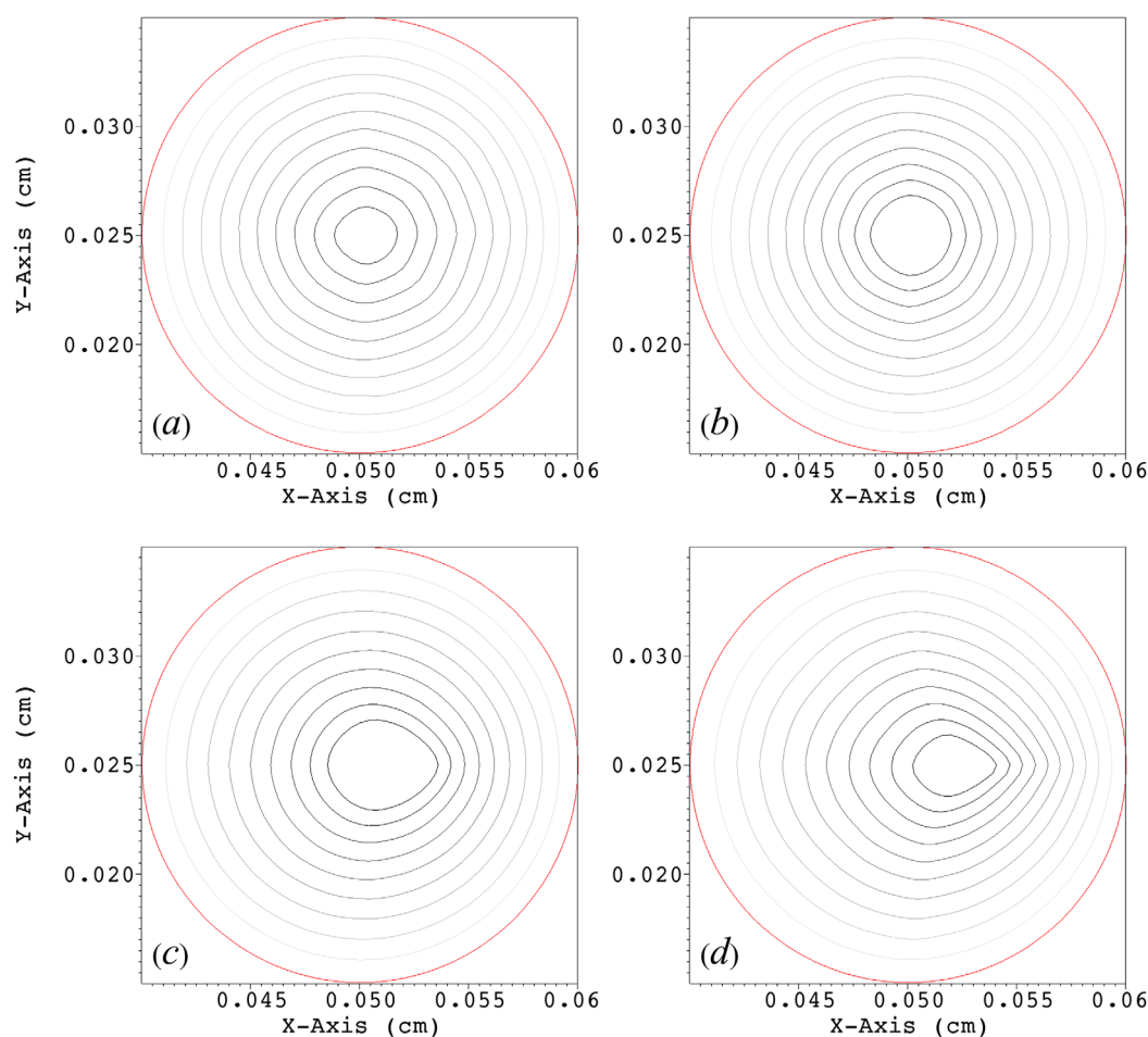
Figure 2. Evolution of a single calcite grain at a range of inlet fluid velocities (a) 0.0012 cm/s, (b) 0.012 cm/s, (c) 0.12 cm/s, and (d) 1.2 cm/s. In red is the original grain boundary, and later stages are shown as a gray scale with increasing shade with time.
